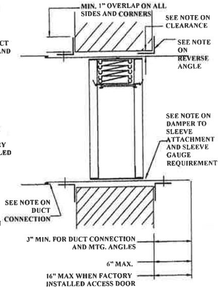
WALL MOUNT SHOWN (VERTICAL INSTALLATION)
