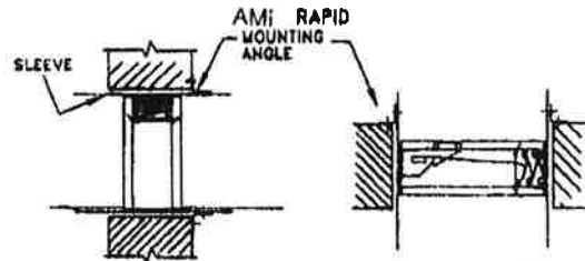
HORIZONTAL INSTALLATION AMi RAPID MOUNTING ANGLE MUST BE INSTALLED ON TOP OF FLOOR.
