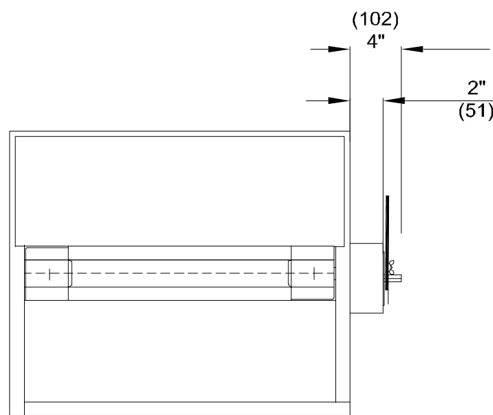
2" (51) hand quadrant stand-off bracket SINGLE BLADE (UP TO 36" X 12")
