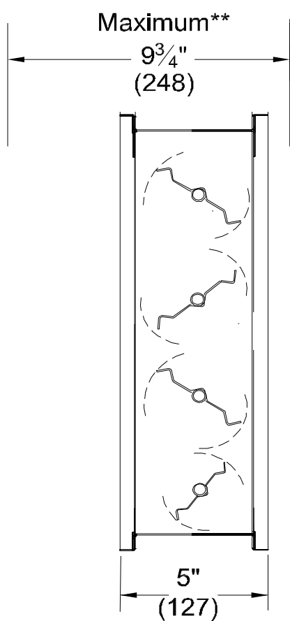
OPPOSED BLADE
